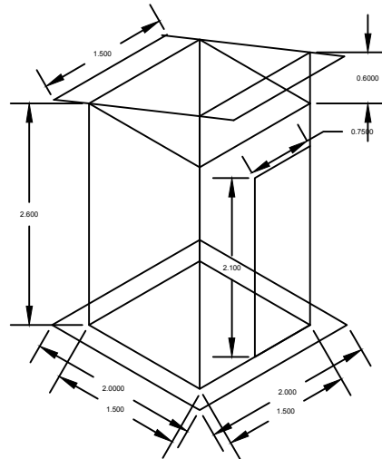
3D MODEL VIEW (TOILET)
